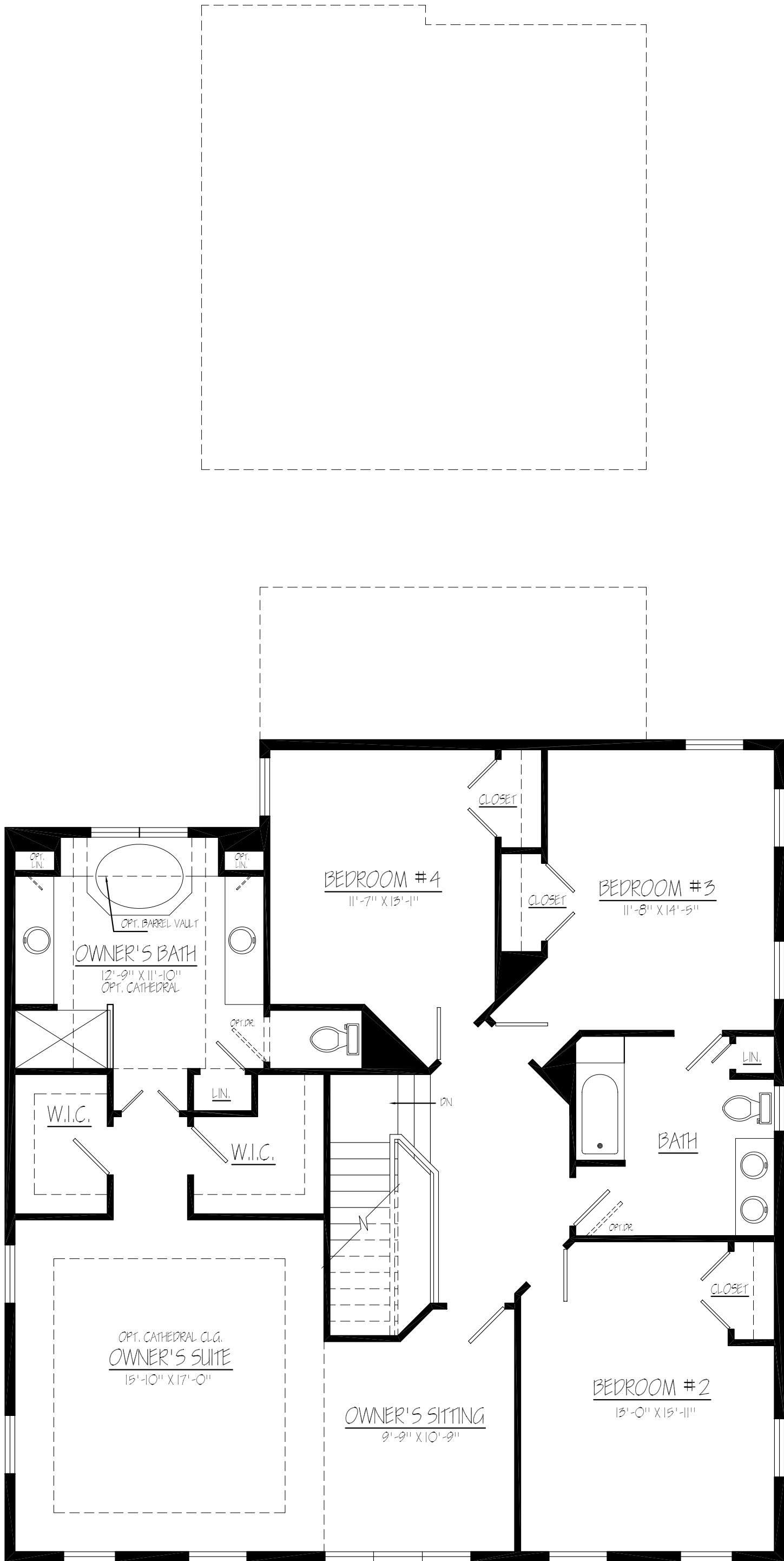
○ SECOND FLOOR PLAN - NO PORCH SCALE = 3/16" = 1'-0"
