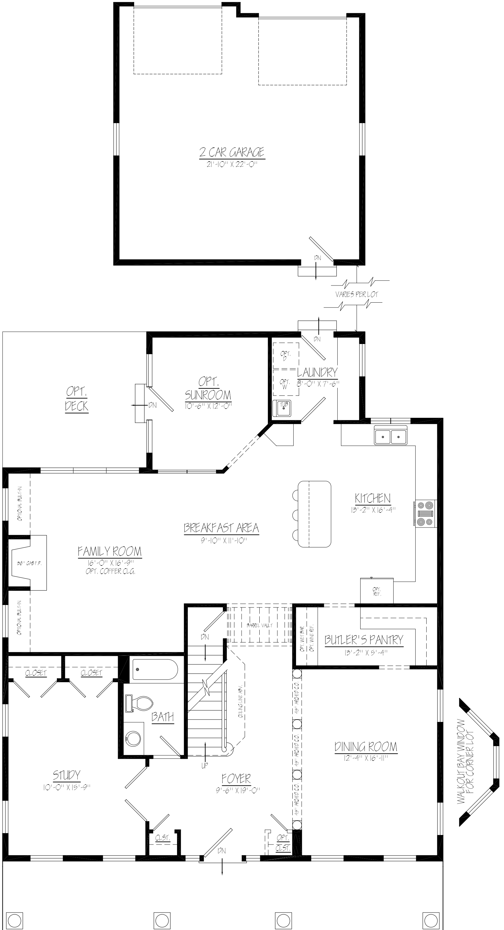
FIRST FLOOR PLAN SCALE = 3/16" = 1'-0"
