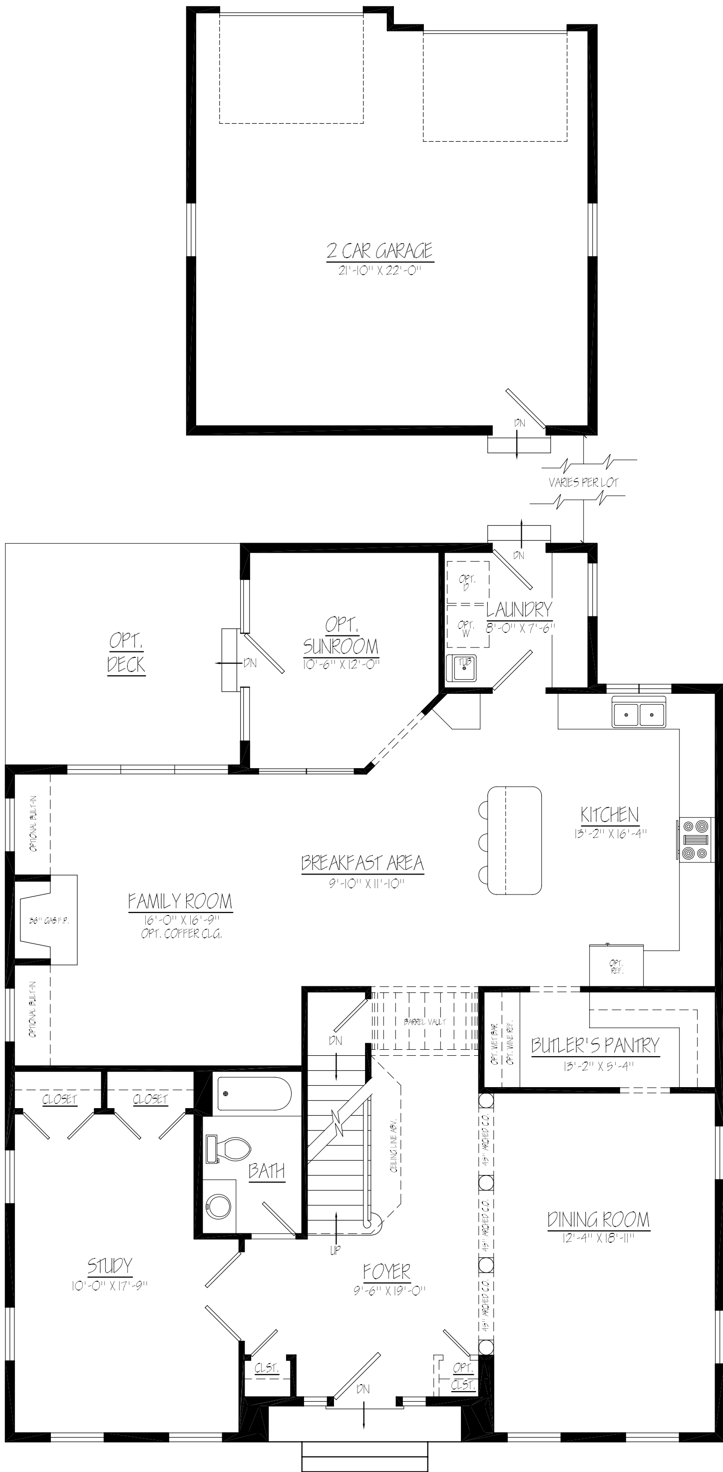
○ FIRST FLOOR PLAN - NO PORCH SCALE = 3/16" = 1'-0"
